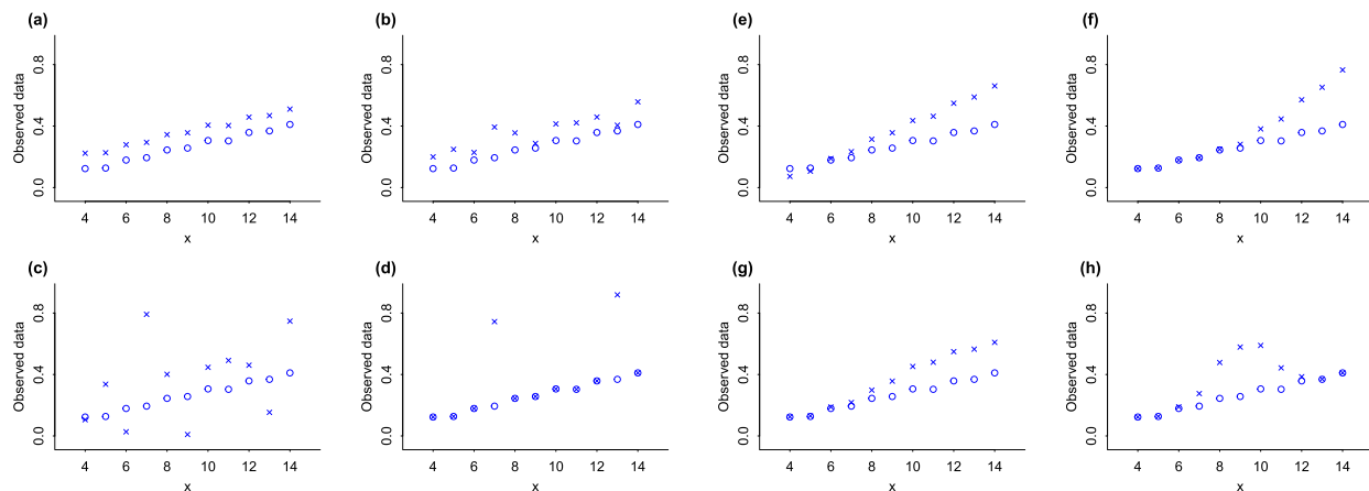
Figure 3. Two quartets showing different patterns of observable data consistent with the causal effects displayed in Figures 1 and 2. In each plot, the crosses and circles represent treated and control units, respectively, and the difference between the two is the treatment effect.
