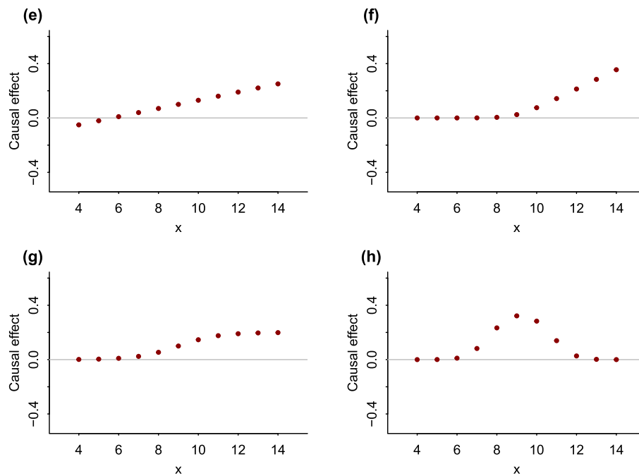
Figure 2. Four graphs showing patterns of causal effects, each with average effect of 0.1, but varying in different ways as a function of a pretreatment predictor: (e) linear interaction, (f) no effect then steady increase, (g) plateau, (h) intermediate zone with large effects.
