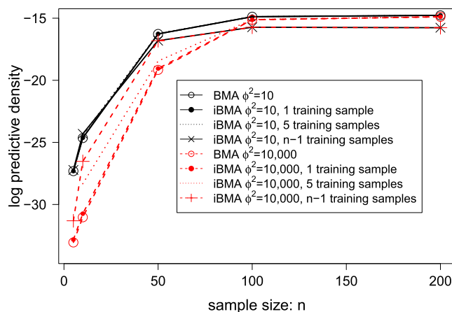
Figure 1: Averages of log predictive densities for 10 test points based on 50 Monte Carlo replicates. Black corresponds to authors' prior, red corresponds to a more vague prior on coefficients. Increasing the training sample size diminishes the effect of the prior but also reduces log predictive density at higher sample sizes. None of the iBMA settings produce predictive densities substantially higher than the BMA approach (open circles).
