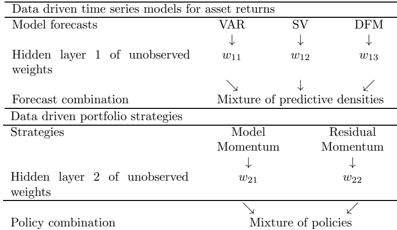
Figure 1: Data driven density combinations and machine learning.
